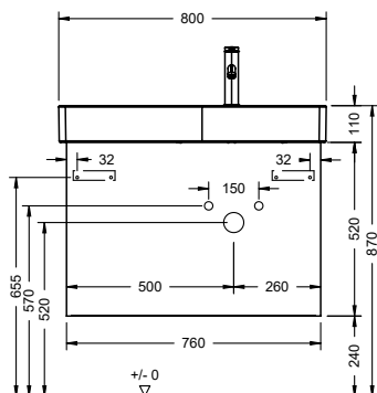
WWLT_WWLS076 passend zu Duravit Durasquare 234980
