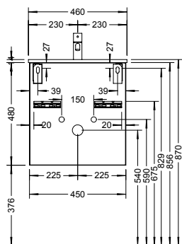
WVAK045 WT 14mm
