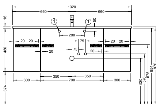
MWEJ132/MWEK132 // WUYN/WUYO070 // WUYP/WUYQ/WUYR030
