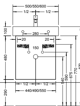
WVNR044 WVNR049 / WVNR055 WVNS049 / WVNS055 WVNT055
